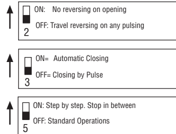
DIP-SWITCH N°3=ON Automatic Closing
