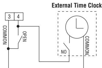
DIP-SWITCH N°3=ON Automatic Closing
